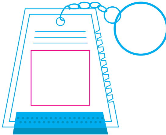
Cyan Line - AA-101 Keytag Ice Scraper (1.98 W x 2.15754 H X 0.125 D) Magenta Line - Imprint Area (1 W x 0.9375 H)
