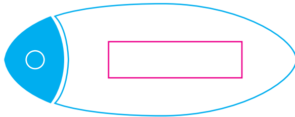
Cyan Line - AA-110 VISOR CLIP (3" W x 1.125" H) Magenta Line - Imprint Area (1.375 W X .375 H)
